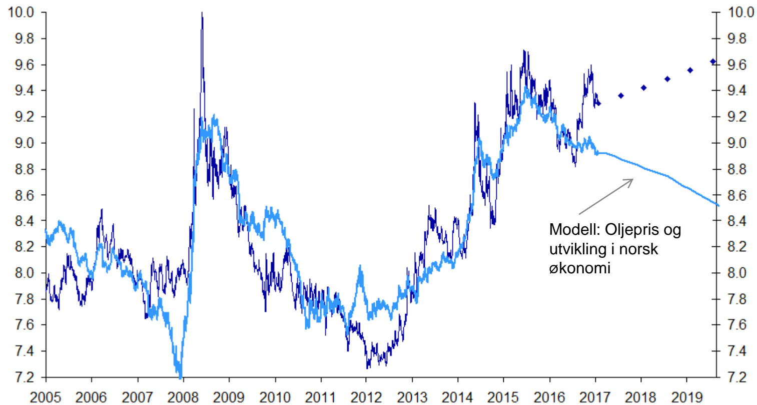
EURNOK model
