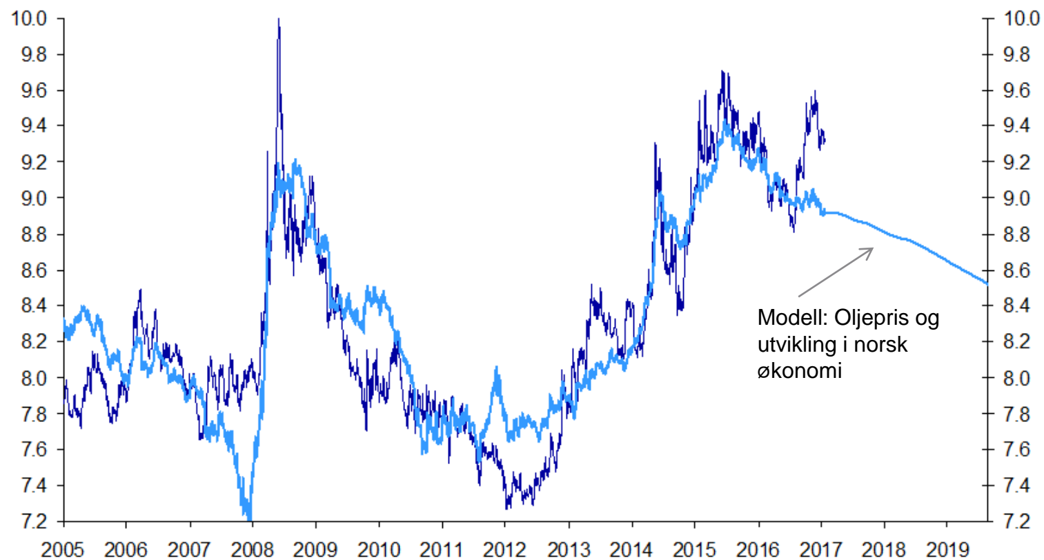
EURNOK model
